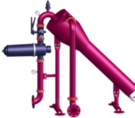
Tekli Plastik Disk Filtreli Seperatörlü Gübreli Filtre Sistemi Separator with Single Plastic Disc Filter System (Fertilizer Apparatus)
