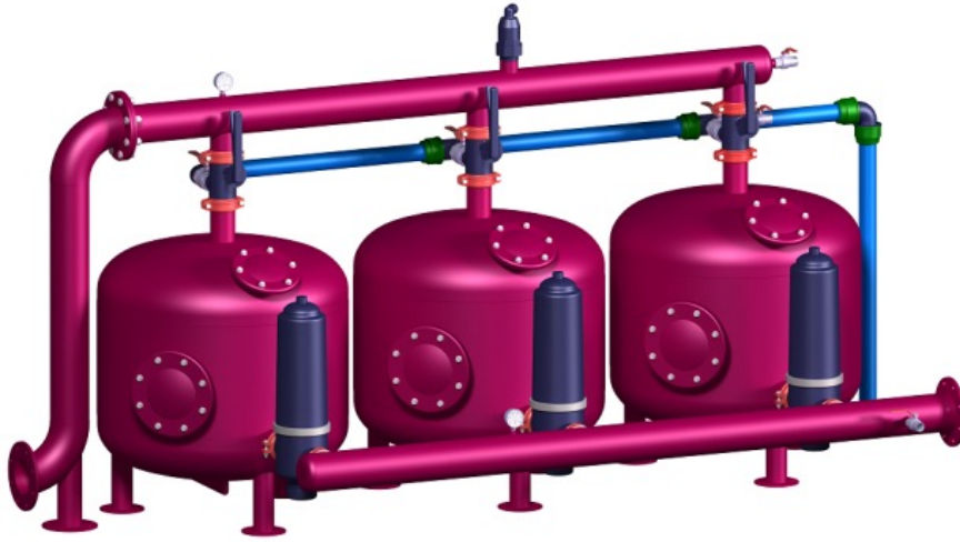
Plastik Disk Filtreli Manuel Geri Yıkamalı Gravel (Yosun) Filtre Sistemi Gravel (Media) Manual Self Cleaning Filter System With Plastic Disc Filter
