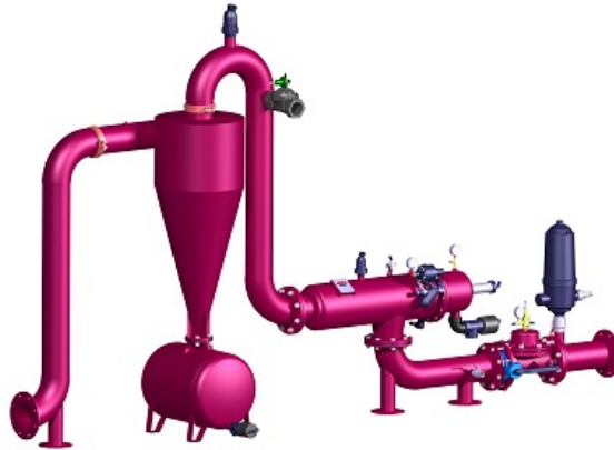
Hidrolik Filtre Hidrosiklonlu Gübreli Sistem Eko Model - Kaba Eleksiz Model Hydraulic Filter System With Hydrocyclone & Fertilizer Apparatus (Eco Model - Without Coarse Screen)
